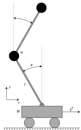
Figure 1: Double Inverted Pendulum System[1]
